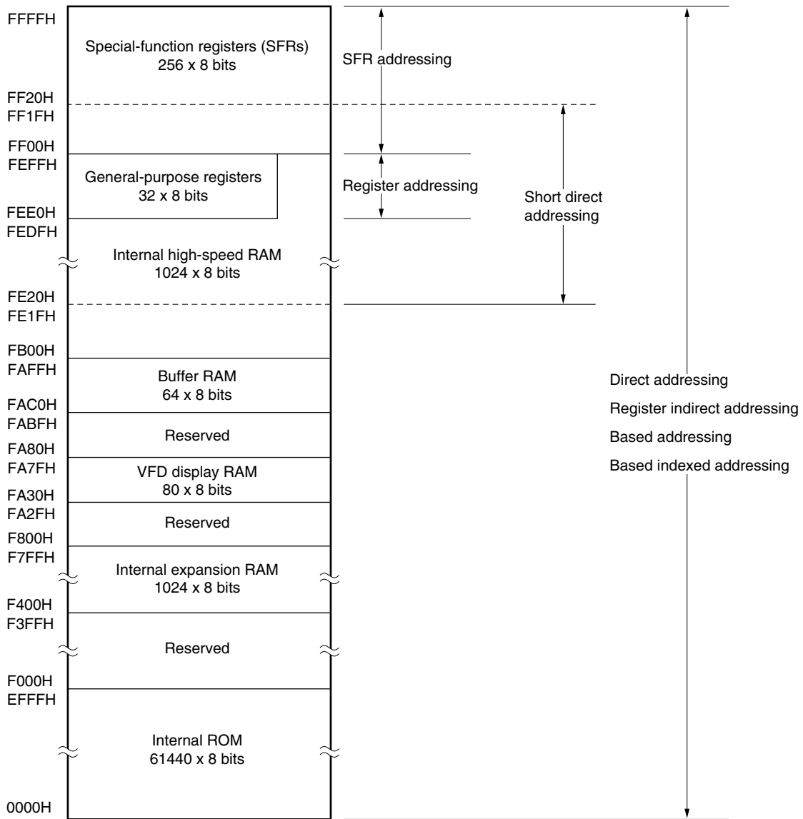
Figure 3-9. Data Memory Addressing ( \mu PD780208)
