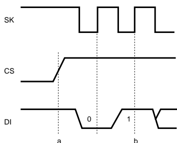
Fig. 8 Erroneous operation timing
