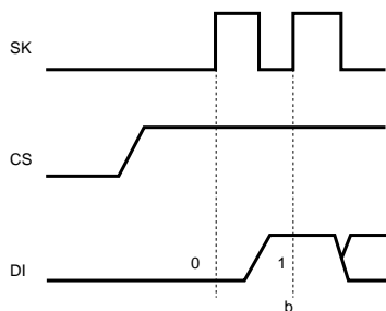
Fig. 9 Normal operation timing
