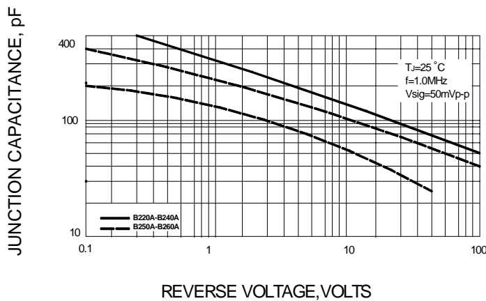
FIG.5-TYPICAL JUNCTION CAPACITANCE
