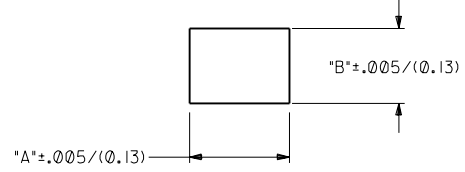
RECOMMENDED HOLE CUTOUT
