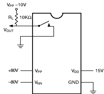
T_{ON}/T_{OFF}
