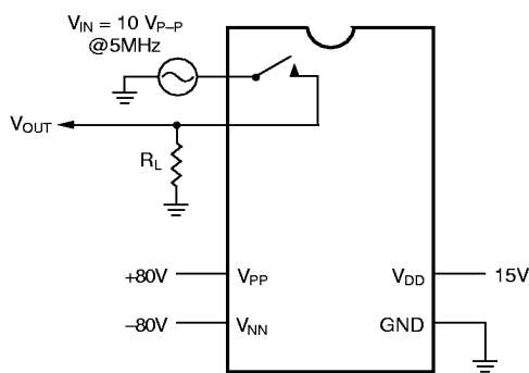
OFF Isolation
