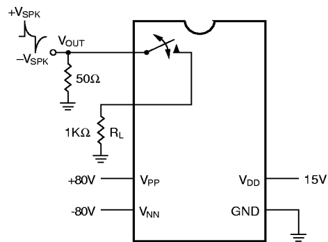
Output Voltage Spike
