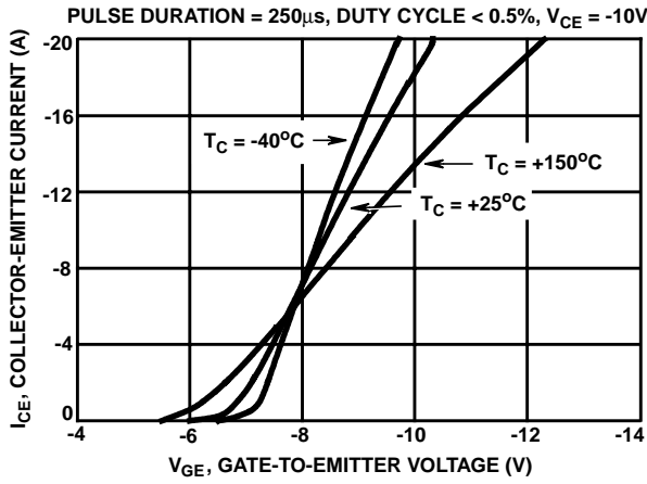
FIGURE 1. TRANSFER CHARACTERISTICS
