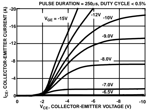
FIGURE 2. SATURATION CHARACTERISTICS
