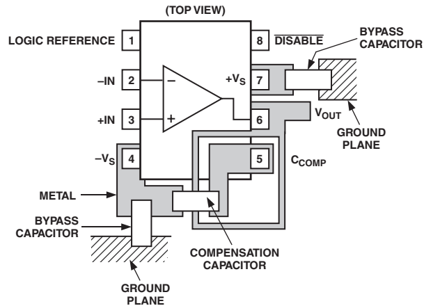
Figure 7. Recommended Location of Critical Components and Guard Ring
