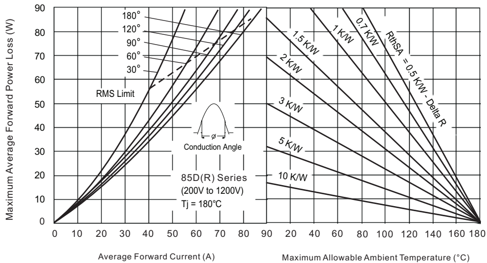
Fig.5 Forward Power Loss Characteristics
