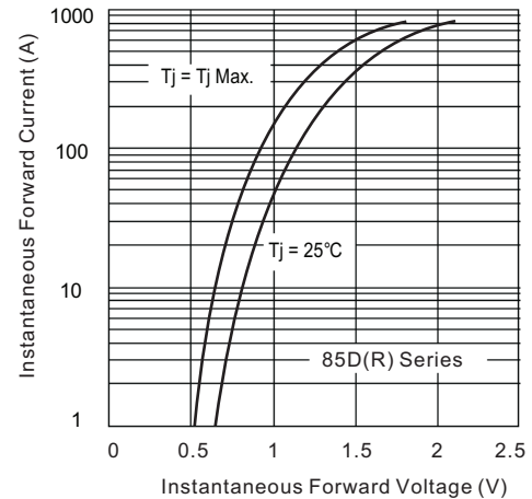
Fig.12 Forward Voltage Drop Characteristics (for 1600V)
