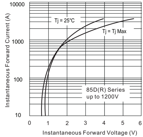
Fig.10 Forward Voltage Drop Characteristics (Up To 1200V)
