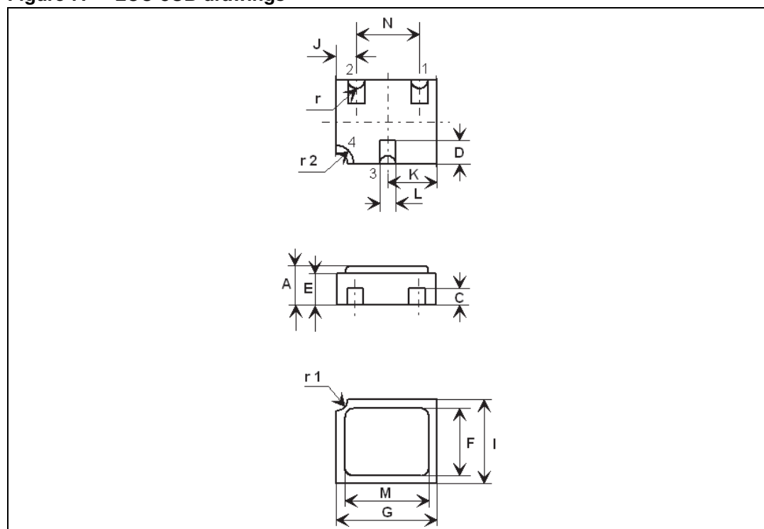
Figure 7. LCC-3UB drawings
