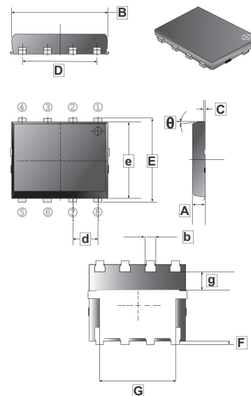
DFN3x3-8PP
