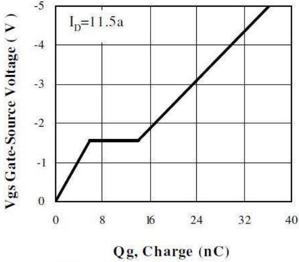
Figure 7. Gate Charge Characteristics
