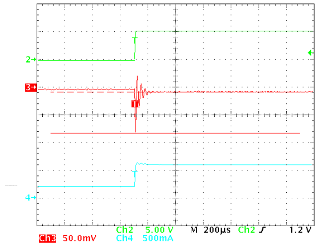
Figure 18. 200 mA to 600 mA Load Transient in 1 \mu\text{s} ( V_{IN} = 3.6 \text{ V} , V_{OUT} = 1.2 \text{ V} , Temperature = 25°C)
