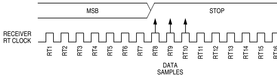
Figure 13-7. Slow Data
