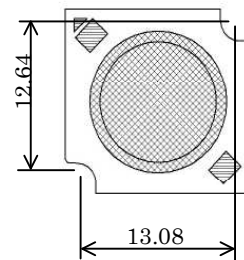
Recommended installation screw pitch
