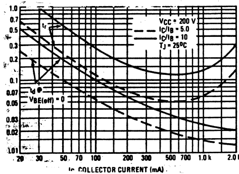
FIGURE 2 – TURN-ON TIME
