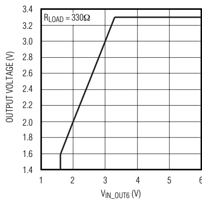
OUT6 REGULATOR LINE REGULATION
