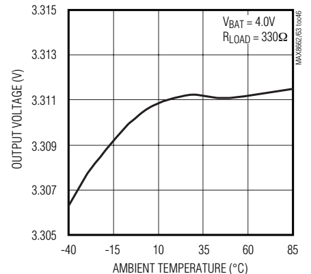
OUT4 VOLTAGE vs. TEMPERATURE
