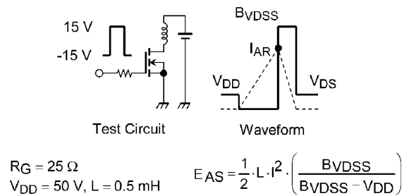
Fig. 8.16 Test Circuit/Waveform
