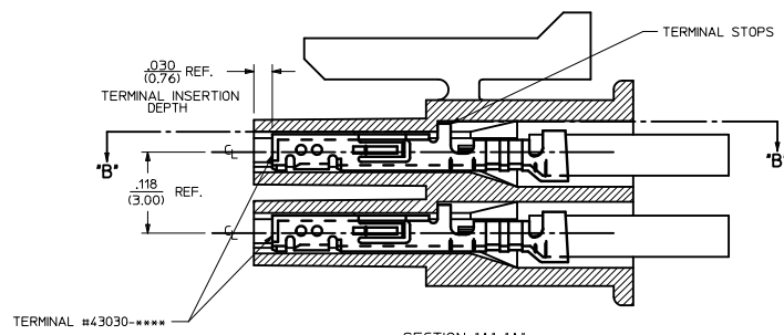
SECTION "A"- "A" WITH TERMINAL (SCALE 10:1)
