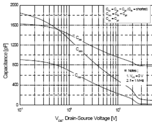
Fig.5 Capacitance Characteristics
