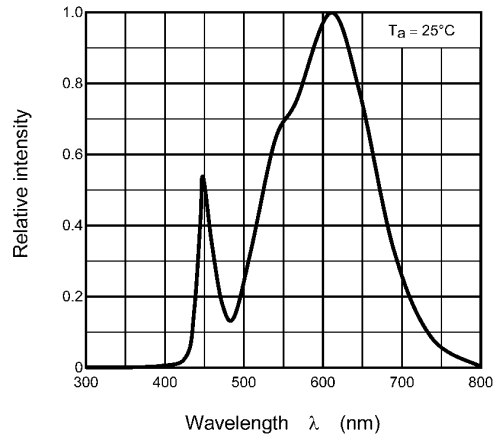
Fig. 8.4 Wavelength characteristic
