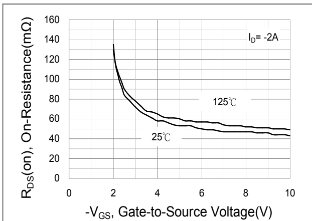
Fig.5 On-Resistance vs. Gate-to-Source Voltage
