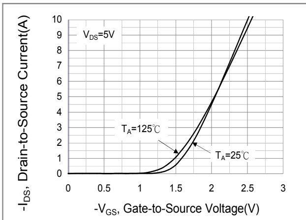
Fig.3 Transfer Characteristic
