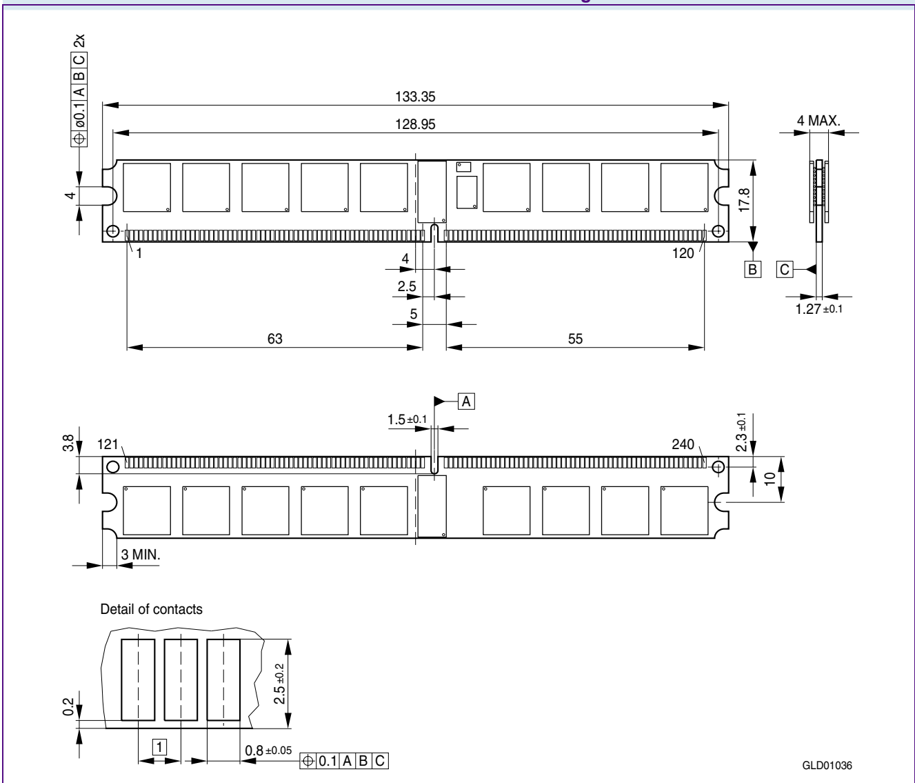
FIGURE 5 Package Outline Raw Card H - L-DIM-240-53
