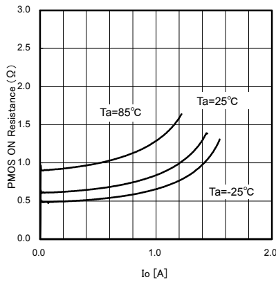
Fig.16. PchFET ON resistance Io property [VCC=4.5V]
