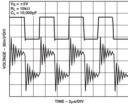
Figure 4. OPA627 Driving C_L = 10,000\text{pF}
