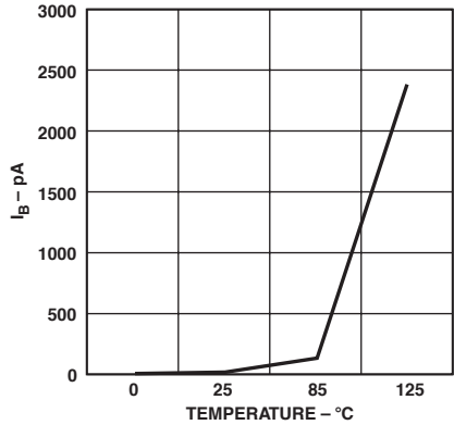
TPC 29. Input Bias Current vs. Temperature
