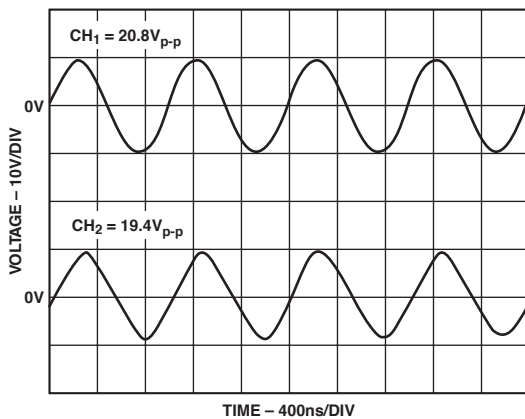
Figure 15. AD8610 FPBW
