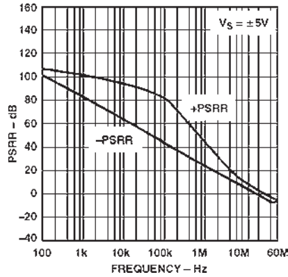
TPC 20. PSRR vs. Frequency at \pm 5\text{ V}
