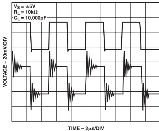
Figure 5. AD8610/AD8620 Driving C_L = 10,000\text{pF}
