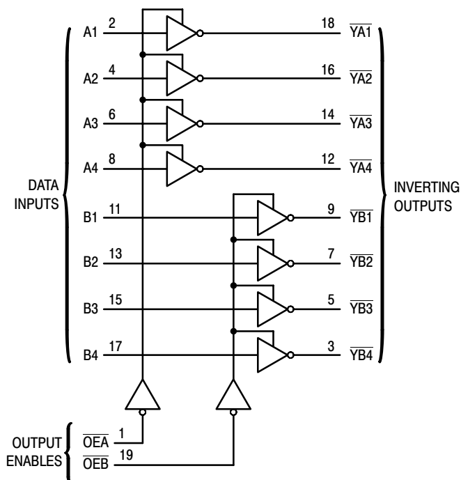
Figure 1. LOGIC DIAGRAM
