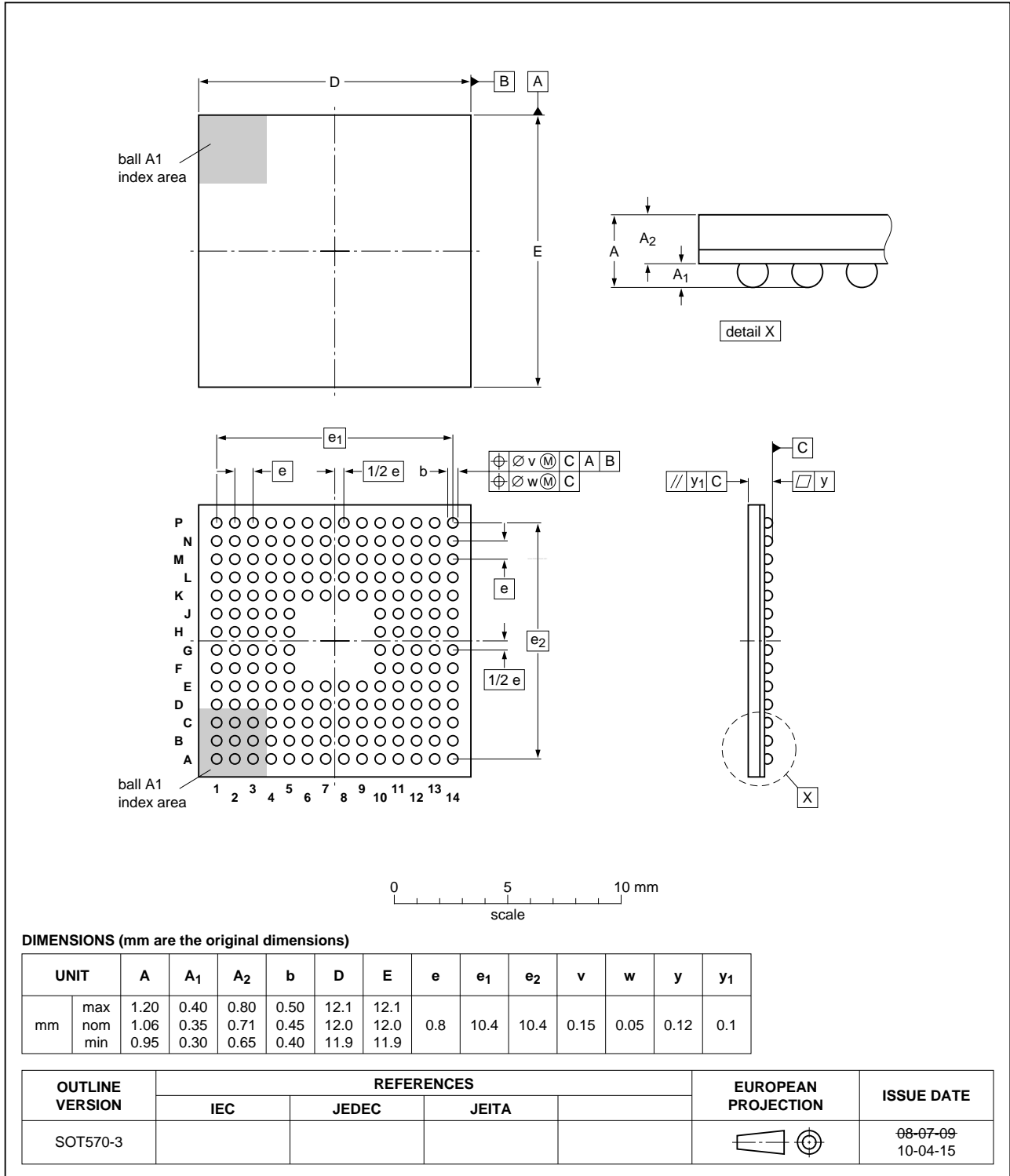
Fig 44. Package outline of the TFBGA180 package
