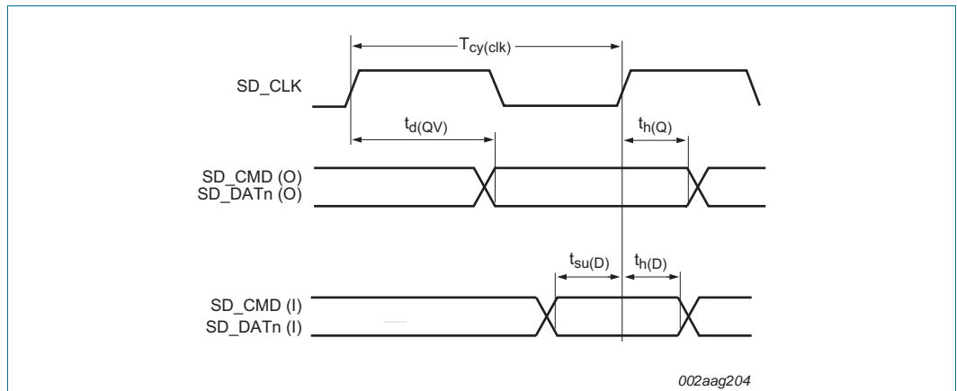
Fig 35. SD/MMC timing
