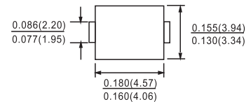
DO-214AA(SMB)
