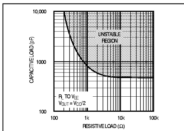
Figure 4. Capacitive-Load Stability
