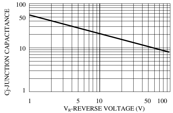
Fig. 4-TYPICAL JUNCTION CAPACITANCE
