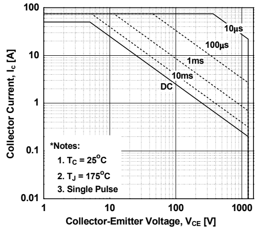
Figure 10. SOA Characteristics
