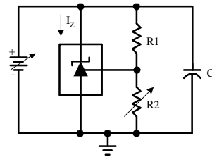
Stability Circuit
