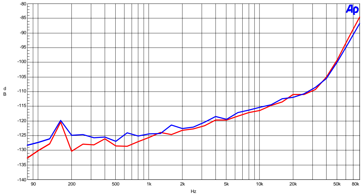
Figure 34. Crosstalk (0dBFS input)
