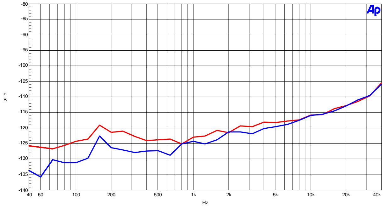
Figure 25. Crosstalk (0dBFS input)
