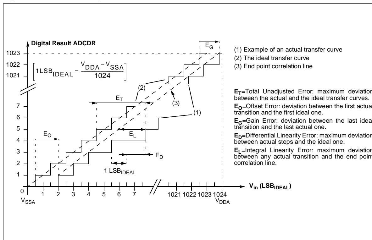
Figure 90. ADC Accuracy Characteristics
