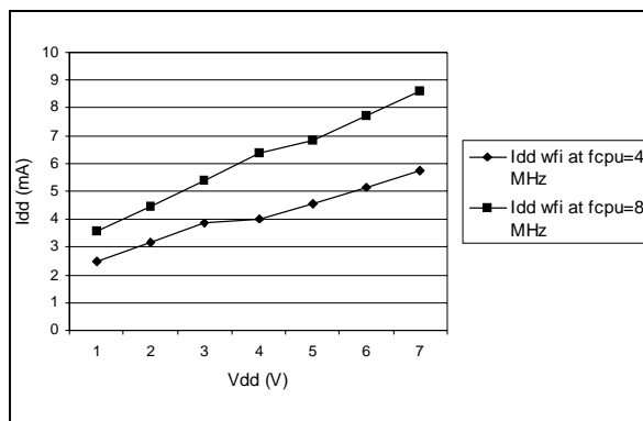
Figure 57. Typ. I_{DD} in WAIT at 4 and 8 MHz f_{CPU}
