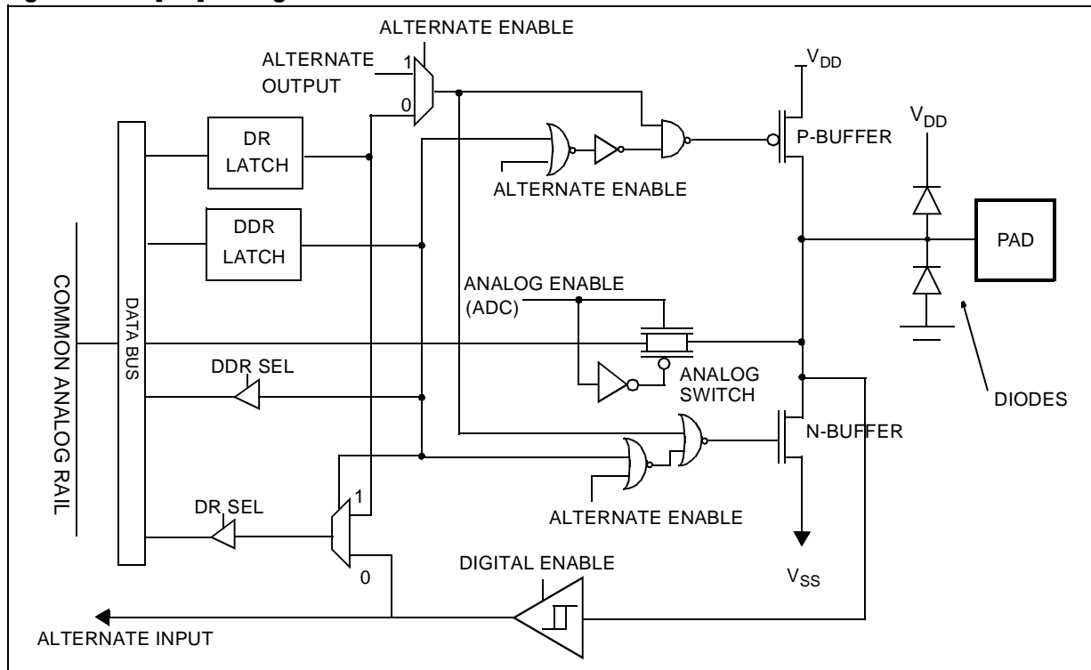
Figure 26. PA[7:0] Configuration
