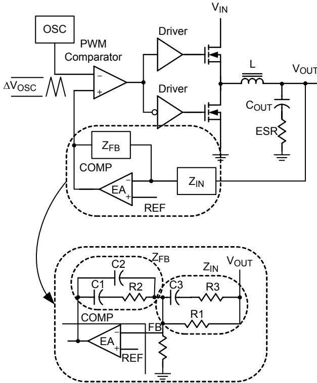
Figure 9. Compensation Circuit
