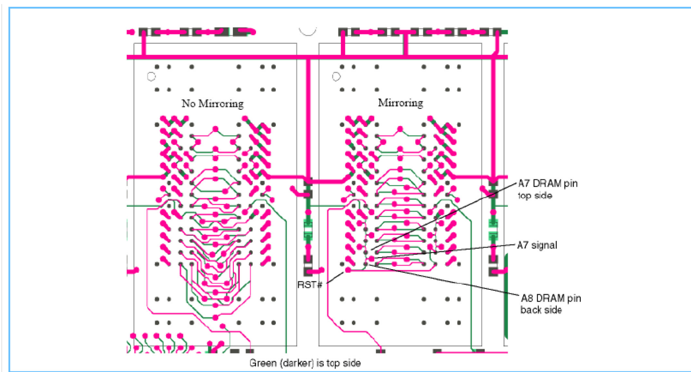
Figure 1. Wiring Differences for Mirrored and Non-Mirrored Addresses
