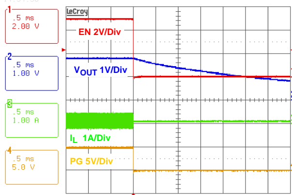
FIGURE 38. SOFT-DISCHARGE SHUTDOWN
