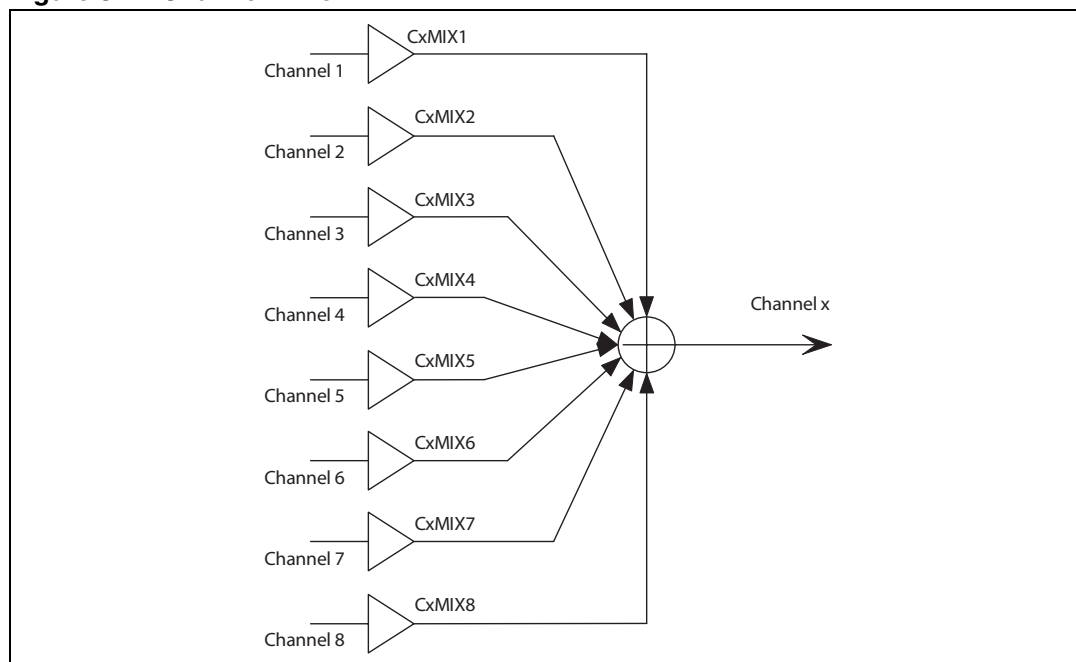
Figure 8. Channel mixer
