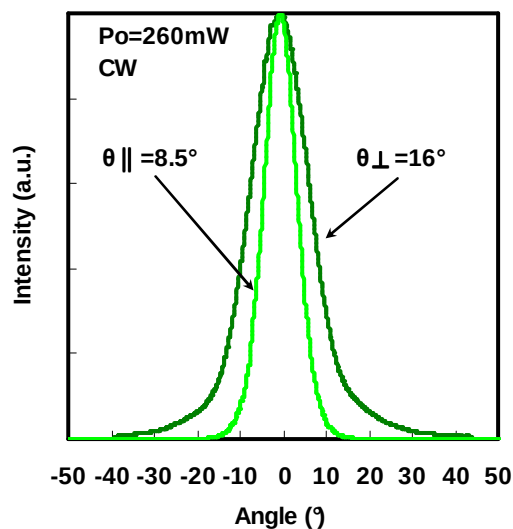
Far-Field-Patterns
