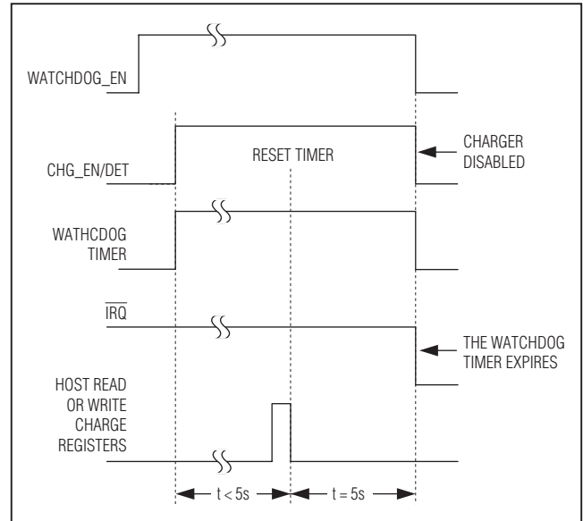
Figure 4. Watchdog Timing Diagram
