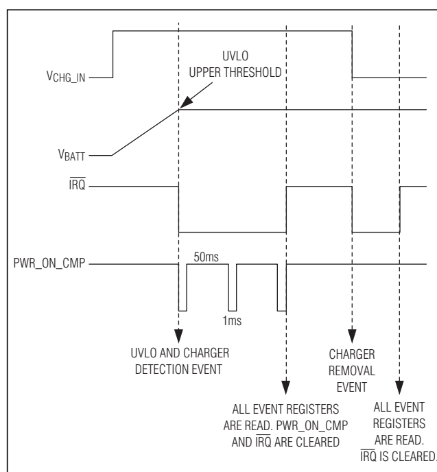
Figure 5. Wake-Up Sequence
