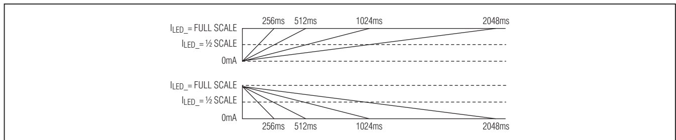
Figure 6. Ramp-Up/Ramp-Down
