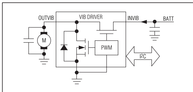
Figure 7. Vibrator Driver
