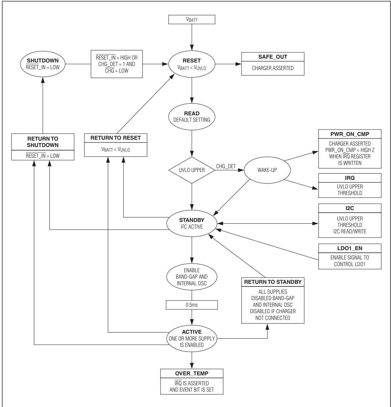
Figure 2. MAX8939 State Diagram
