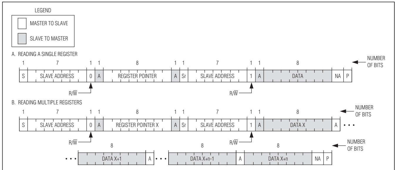
Figure 14. Reading from the MAX8939
