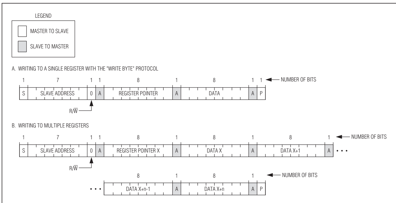
Figure 13. Writing to the MAX8939
