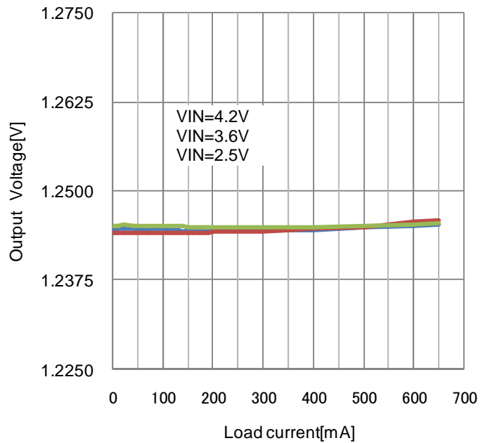
Figure 36. Load regulation PWM mode
