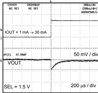
Fig.20 Load Response (Co=1.0 µF) (BH30PB1WHFV)
