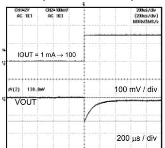
Fig.21 Load Response (Co=1.0 µF) (BH30PB1WHFV)
