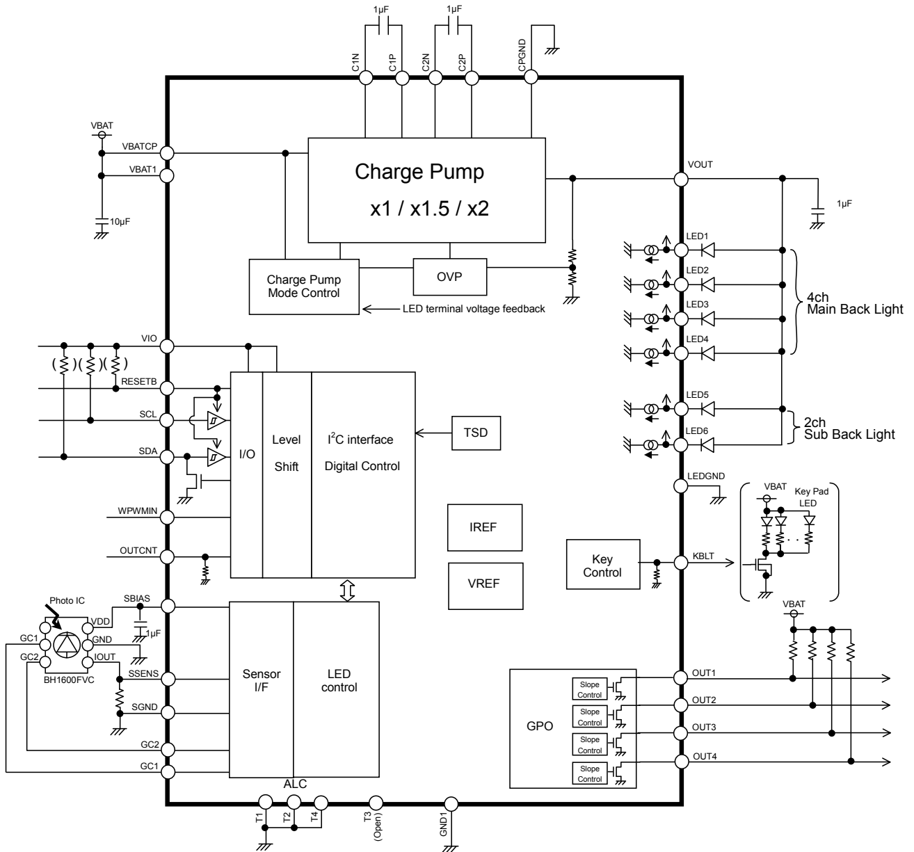
Fig.2 Block Diagram / Application Circuit example 2
