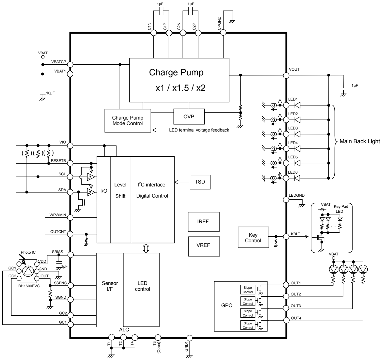
Fig.1 Block Diagram / Application Circuit example 1
