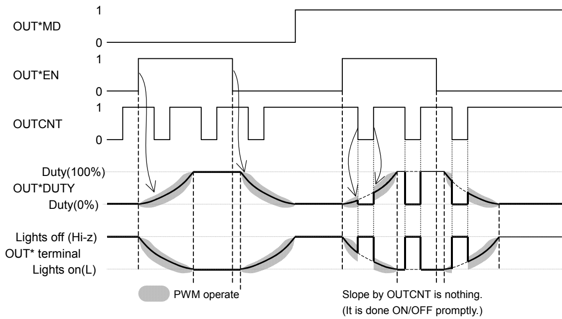
OUT*DUTY show the H section of the output step NMOS gate. (Duty 0%~100 %)
