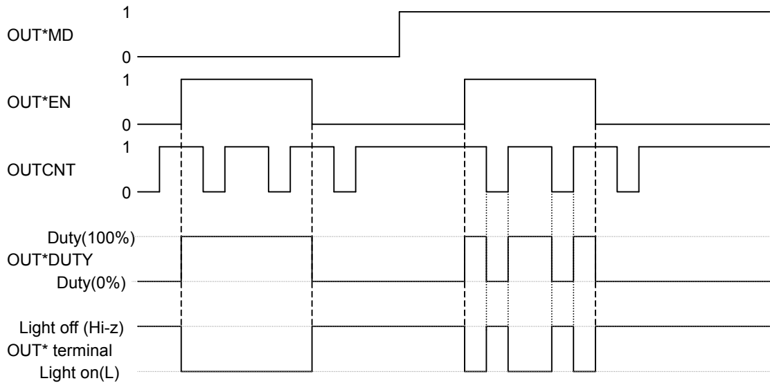
OUT*DUTY shows the H section of the output step NMOS gate. (Duty 0%~100%)
