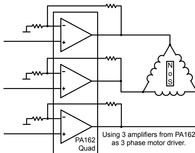
FIGURE 4. 3 Phase Inverter
