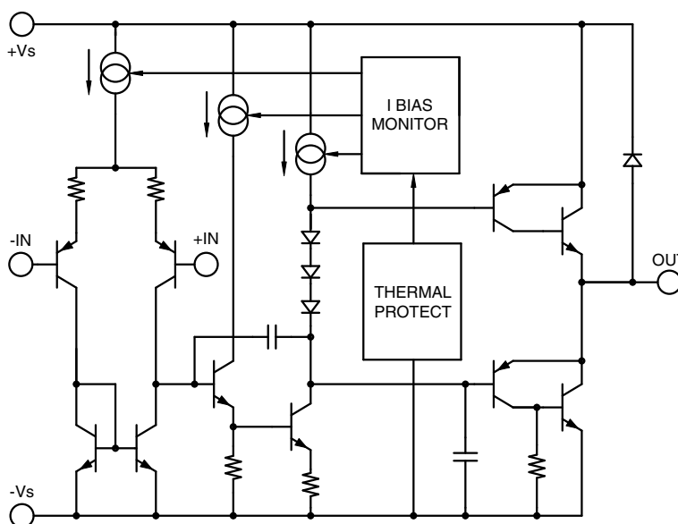
FIGURE 1. Equivalent schematic (one channel)
