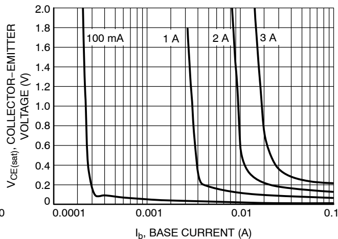
Figure 15. Saturation Region
