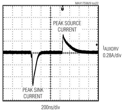
AUXDRV PEAK SOURCE AND SINK CURRENTS
