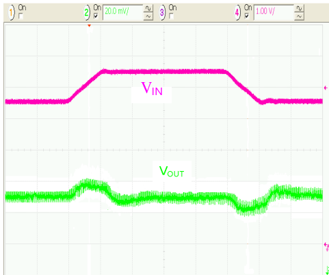
Figure 24. Line Transient Response in PWM Mode, 10 \mu s/div.
