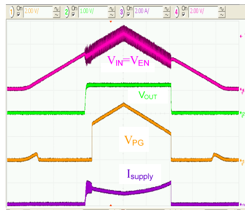
Figure 23. Soft-Start, EN Pin Tied to VCC R_{LOAD}=400m\Omega , C_{OUT}=100\mu F , 1ms/div.
