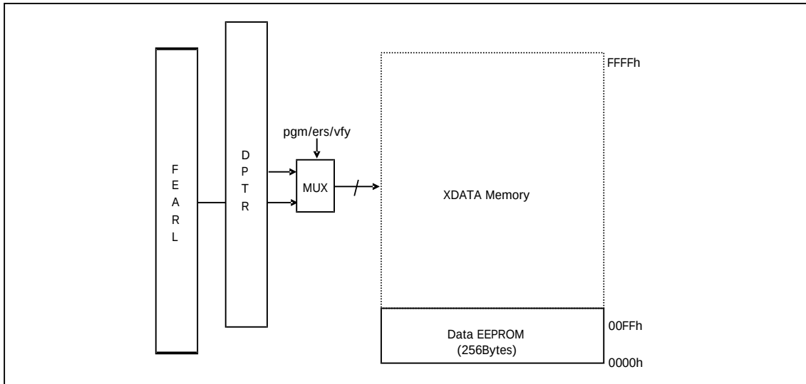
Figure 8.3 Data EEPROM memory map
