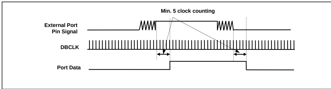
Figure 2.4 Debounce Function
