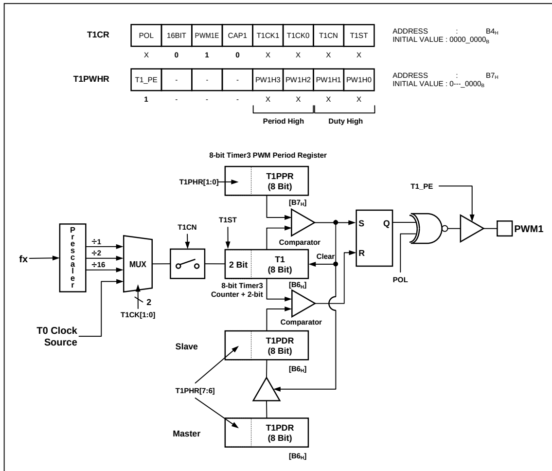
Figure 4.14 PWM Mode
