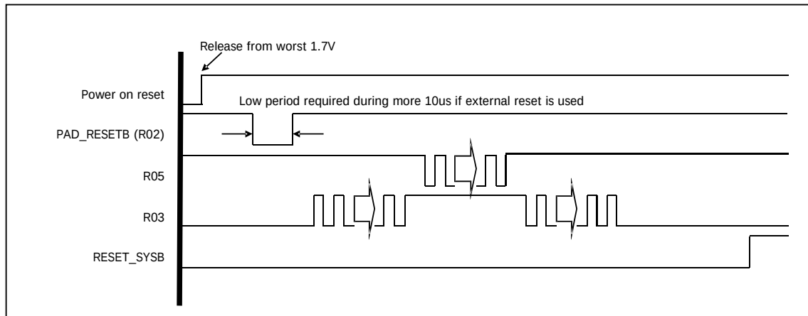
Figure 8.10 ISP mode
