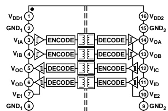
Figure 3. ADuM3402 Functional Block Diagram
