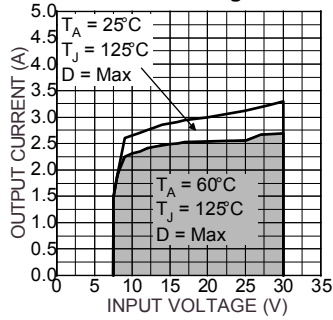
Typical 5V Output SOA Standard Configuration
