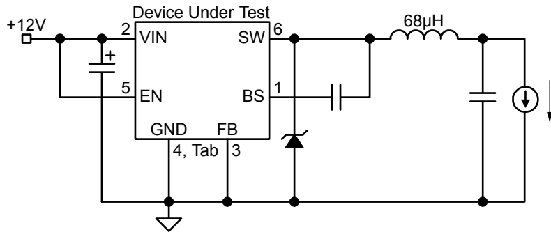
Current Limit Test Circuit
