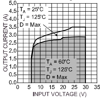
Typical 3.3V Output SOA Standard Configuration
