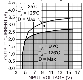
Typical 3.3V Output SOA Bootstrap Configuration
