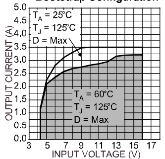
Typical 1.8V Output SOA Bootstrap Configuration
