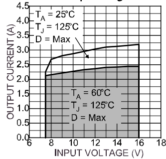
Typical 5.0V Output SOA Bootstrap Configuration
