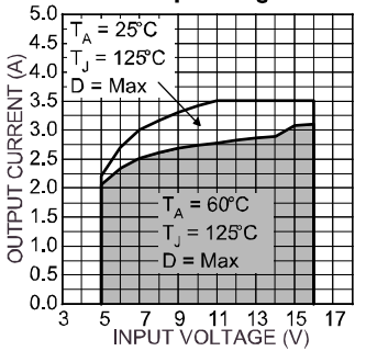
Typical 2.5V Output SOA Bootstrap Configuration
