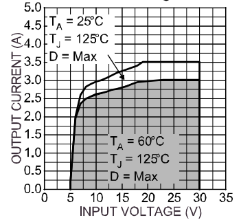
Typical 2.5V Output SOA Standard Configuration
