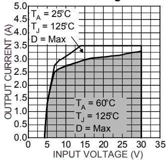
Typical 1.8V Output SOA Standard Configuration
