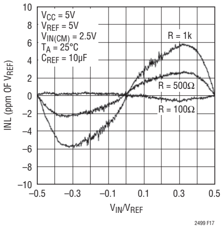
Figure 17. INL vs Differential Input Voltage and Reference Source Resistance for C_{REF} > 1\mu F
