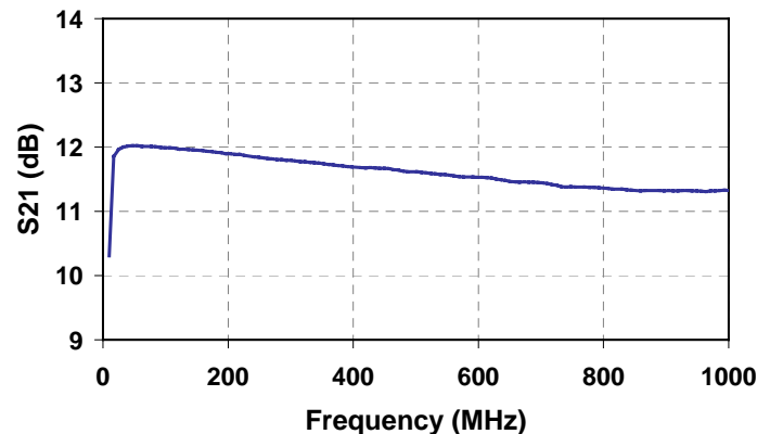
TGA2801B Gain
